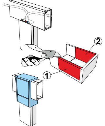
"T" angle
