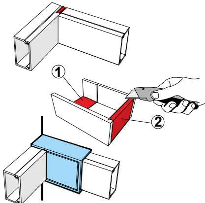
Interior angle
